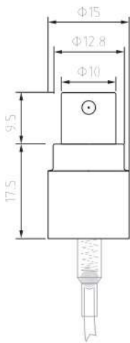
Sprayer
